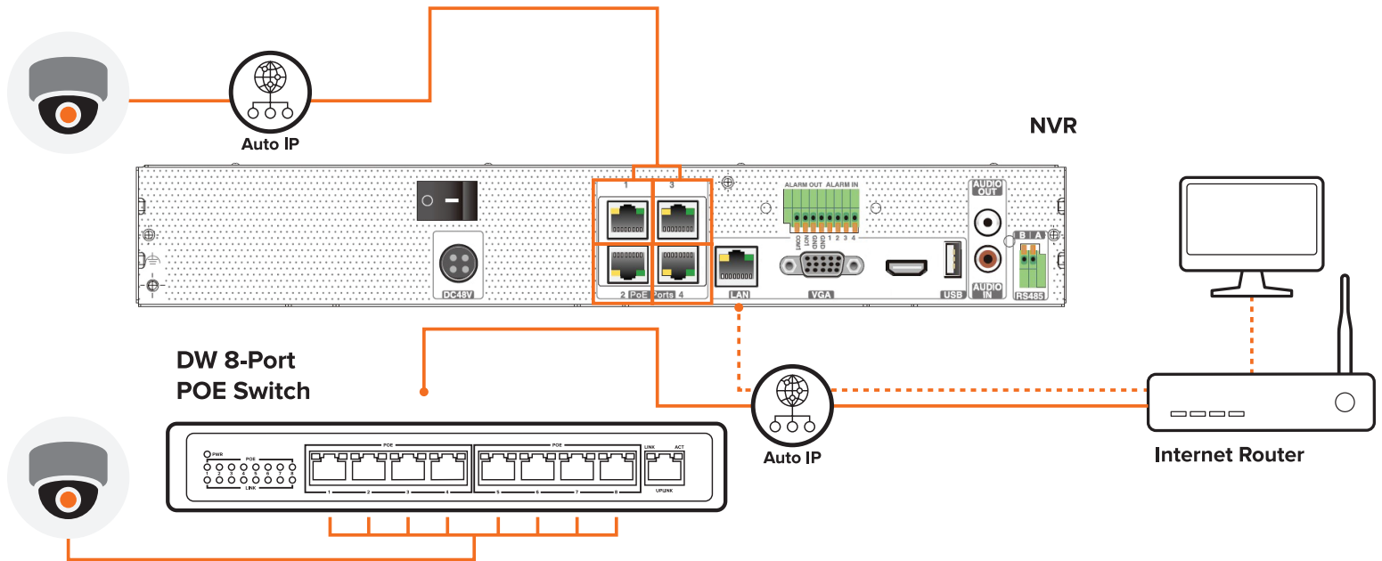
Figure 2. Connecting up to nine (9) cameras with 8-port POE Switch.
