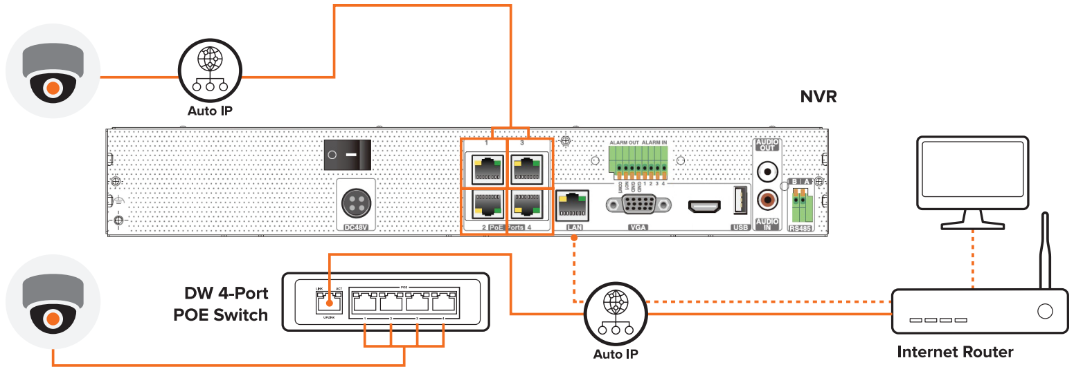
Figure 1. Connecting up to eight (8) cameras with 4-port POE Switch.
